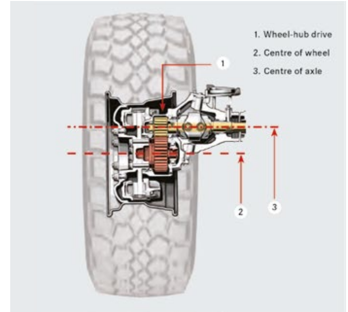
Ample ground clearance due to two identical portal axles with wheel-hub drive.
