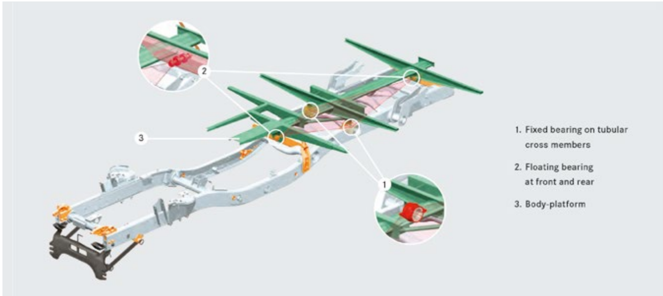
Twist and strain-free mounting of sensitive units and superstructures due to double three-point mounting.
